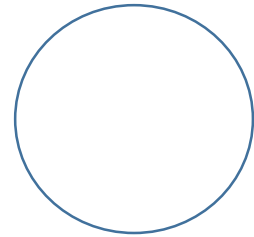
Waxing Gibbous
