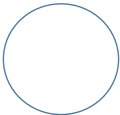
Waning Gibbous
